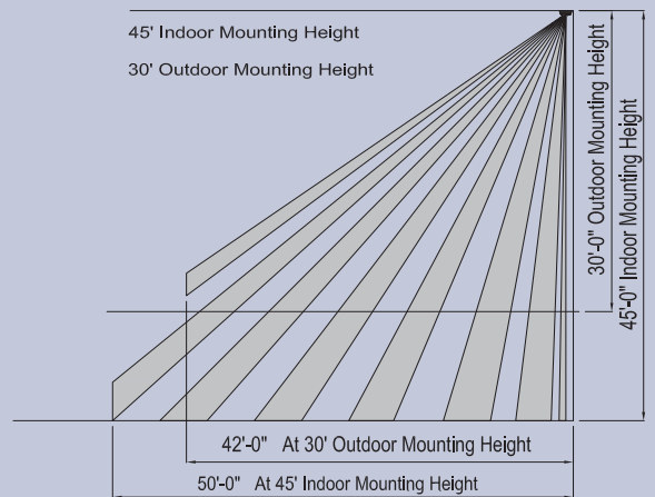
Sensor Lens Coverage and Detection Patterns When Mounted at 30ft and 45ft with Standard Lens
